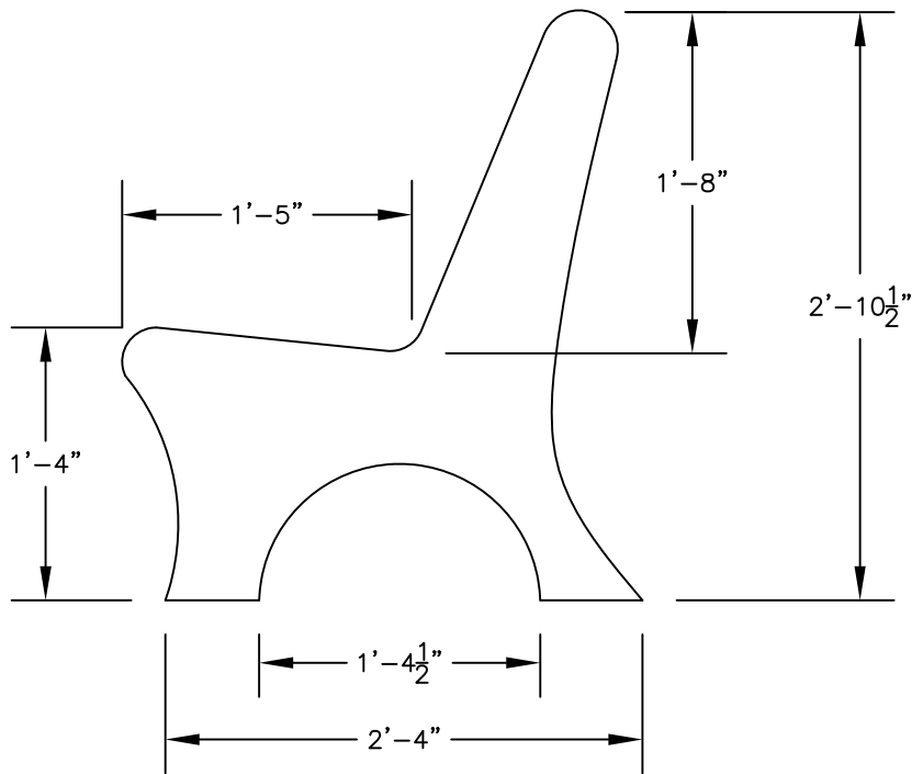
SIDE VIEW
