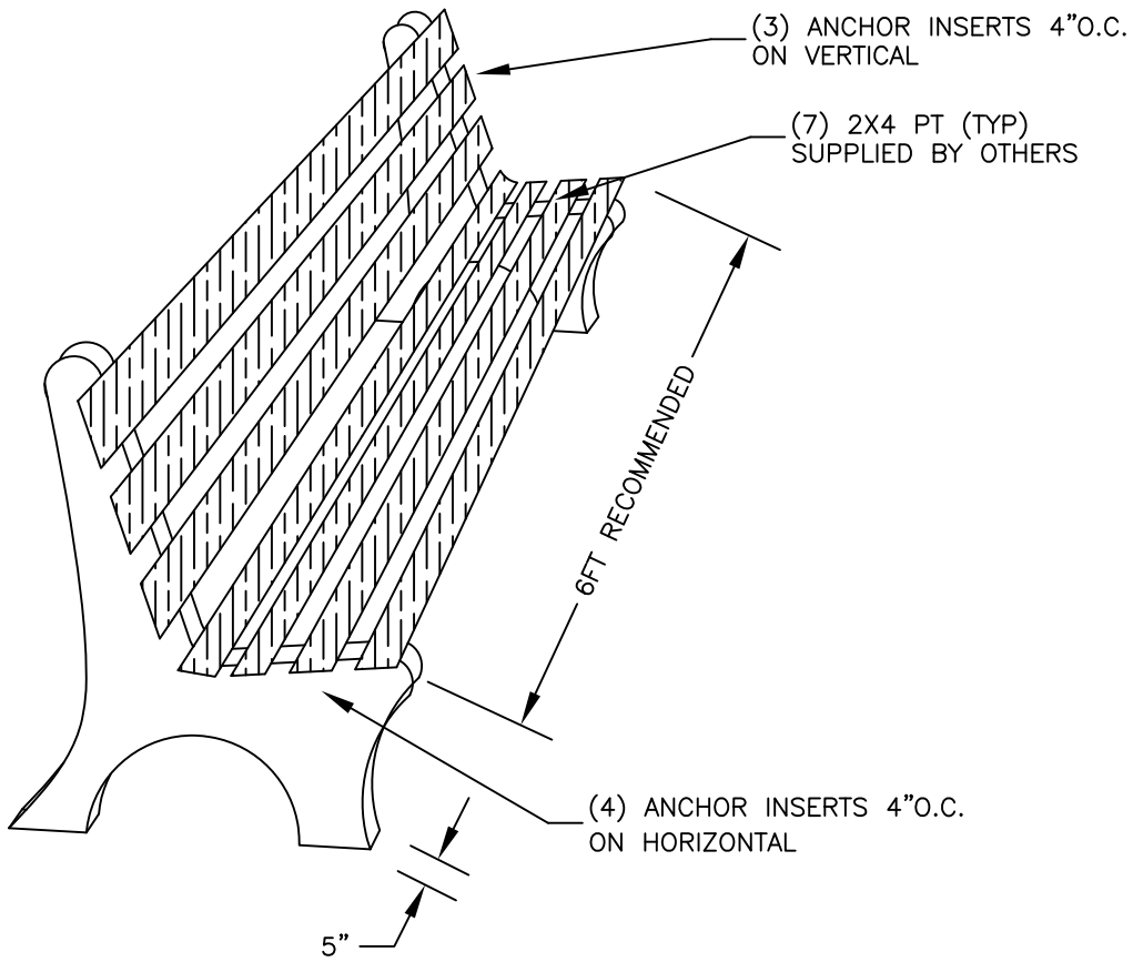
ISO VIEW
